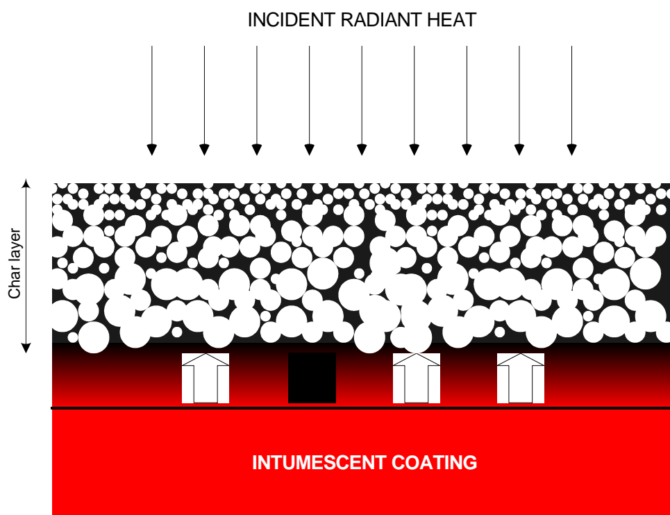
Figure 1 Mechanisms for intumescent systems.
